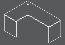
workstation 1700 X 1200 X 600 lefthand CWS17X12X6LH
