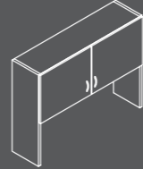
hutch 1150W X 900H X 300D (2 door) CH122D
