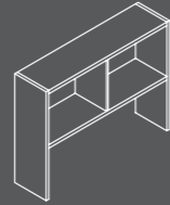
hutch 1150W X 900H X 300D CH12
